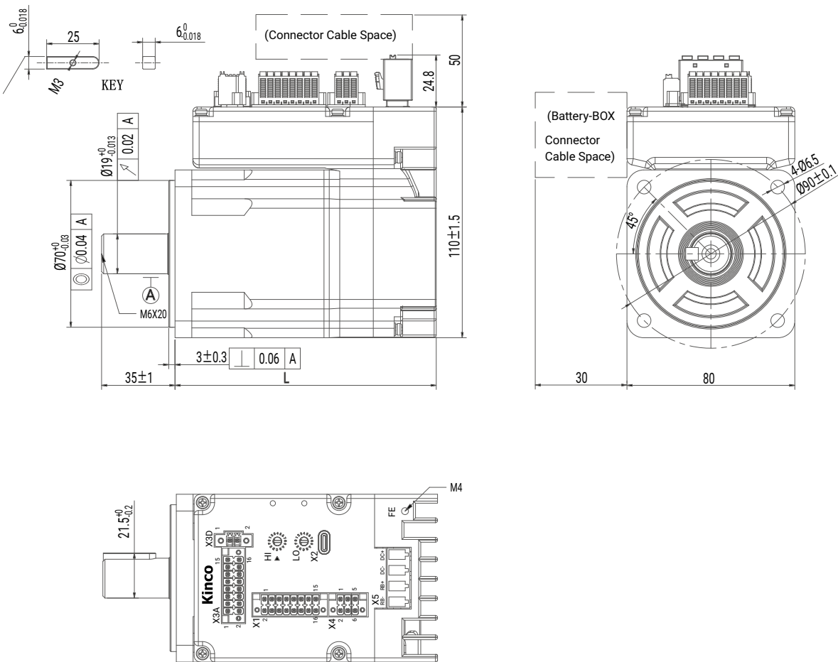
Note:iSMD80D-AA model without X4 port.
